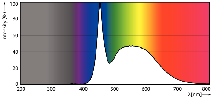
Spectral Power Distribution Colour - TForce Core HB 40W E27 865 WV G3
