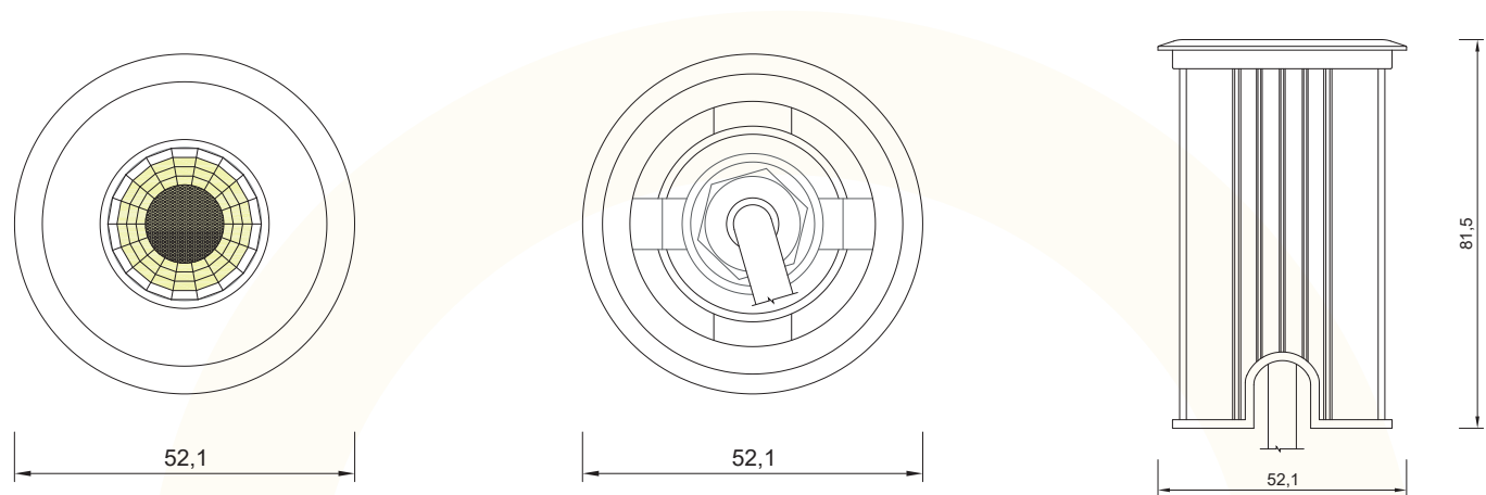
SPOT LED DE PISO INTEGRADO 3W
