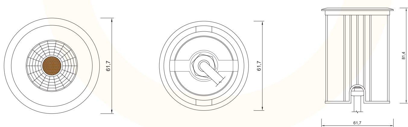
SPOT LED DE PISO INTEGRADO 6W
