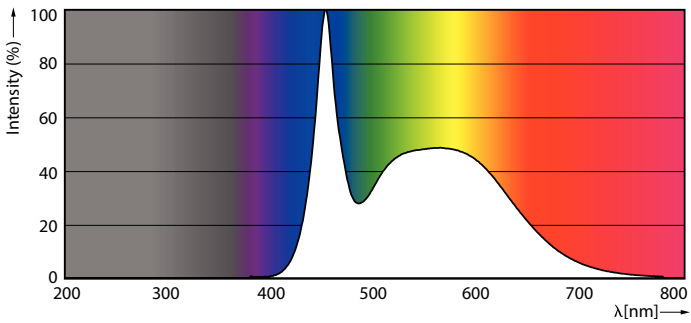
Spectral Power Distribution Colour - TForce Core HB 5Klm 50W E27 865 WV
