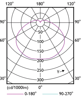
Light Distribution Diagram - TForce Core HB 5Klm 50W E27 865 WV
